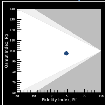
TM-30-20 Rf,Rg
