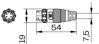
Connector SCALE 1:3
