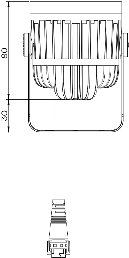
Fixture SCALE 1:2
