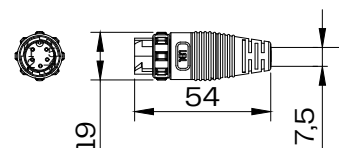
Connector
