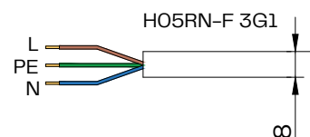
Power cable
