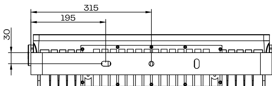
Mounting bracket
