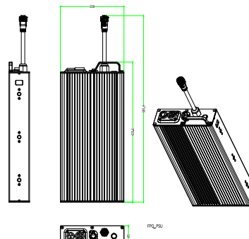
FPQ PSU - Alimentation 750W
