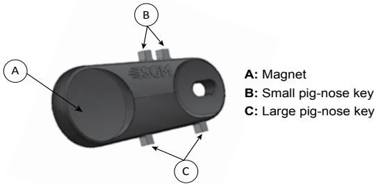
Figure 16: POI Spanner
