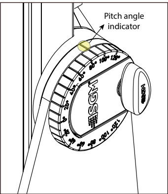
Figure 5: Tilt lock
