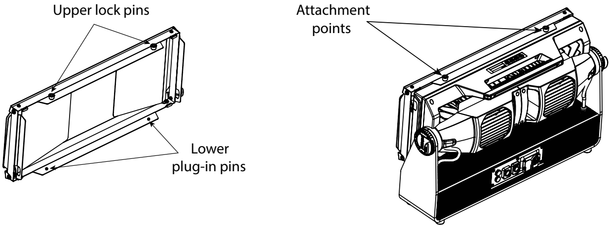
Figure 20: Barndoors
