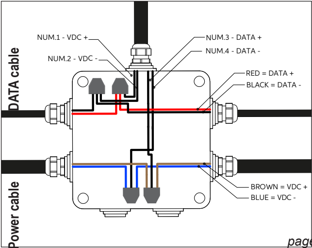
Connection Detail - Separate Cables Connection
