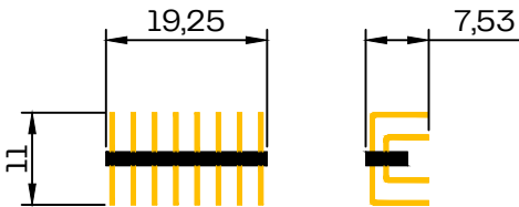
Jumper SCALE 1:1
