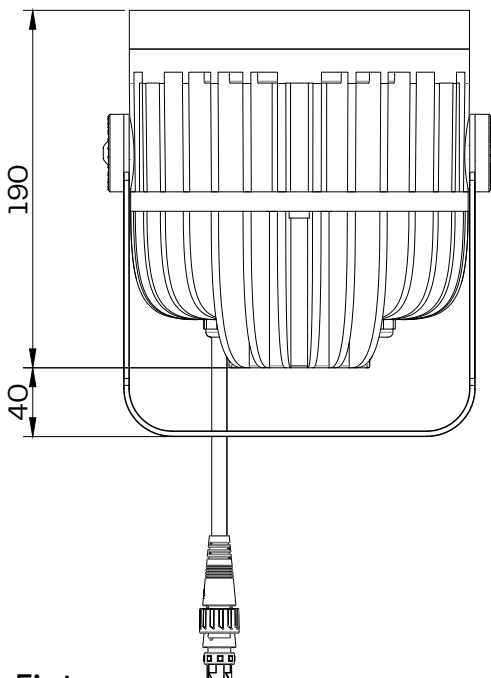
Fixture SCALE 1:4
