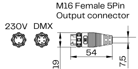
Connector SCALE 1:3
