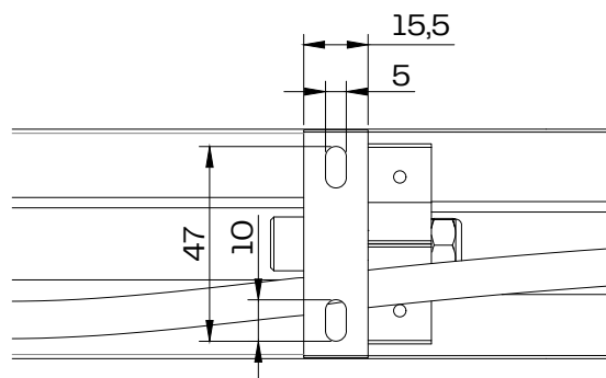
Mounting bracket SCALE 1:2
