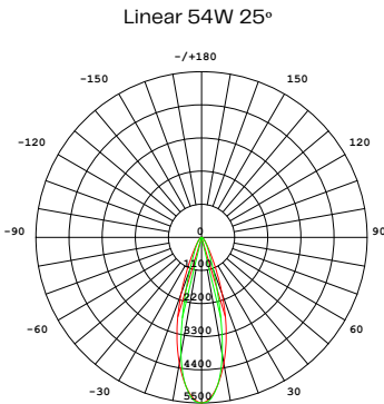
Average Beam angle: 30.2 Deg
