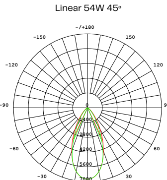
Average Beam angle: 48.1 Deg
