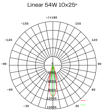
Average Beam angle: 20.5 Deg
