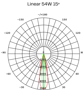
Average Beam angle: 17.6 Deg
