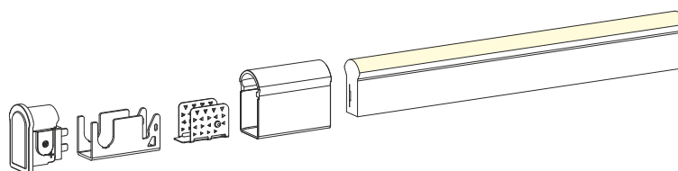
Explosive View / Explosionsansicht
